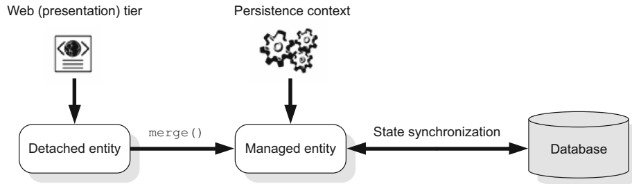
Figure 10.8 An entity instance can be detached and serialized to a separate tier where the client makes changes to the entity and sends it back to the server. The server can use a merge operation to attach the entity to the persistence context.
