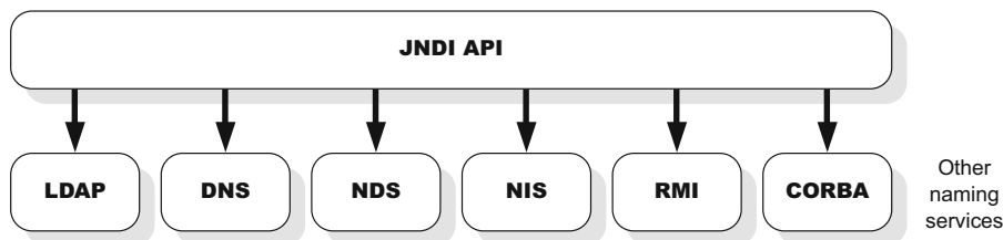
Figure 5.2 JNDI provides a single unified API to access various naming services such as LDAP, DNS, NDS, NIS, RMI, and CORBA. Any naming service with a JNDI SPI provider can be plugged into the API seamlessly.
